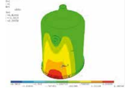
Trunnion of the new FCC Top Part
